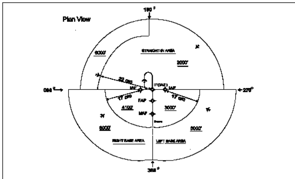
FIG 5-4-8 Sectored TAA Areas
