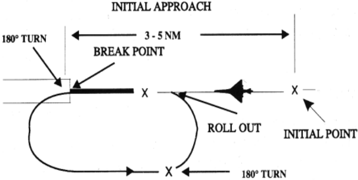
FIG 5-4-27 Overhead Maneuver
