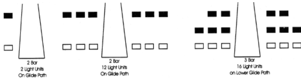
FIG 2-1-4 VASI Variations
