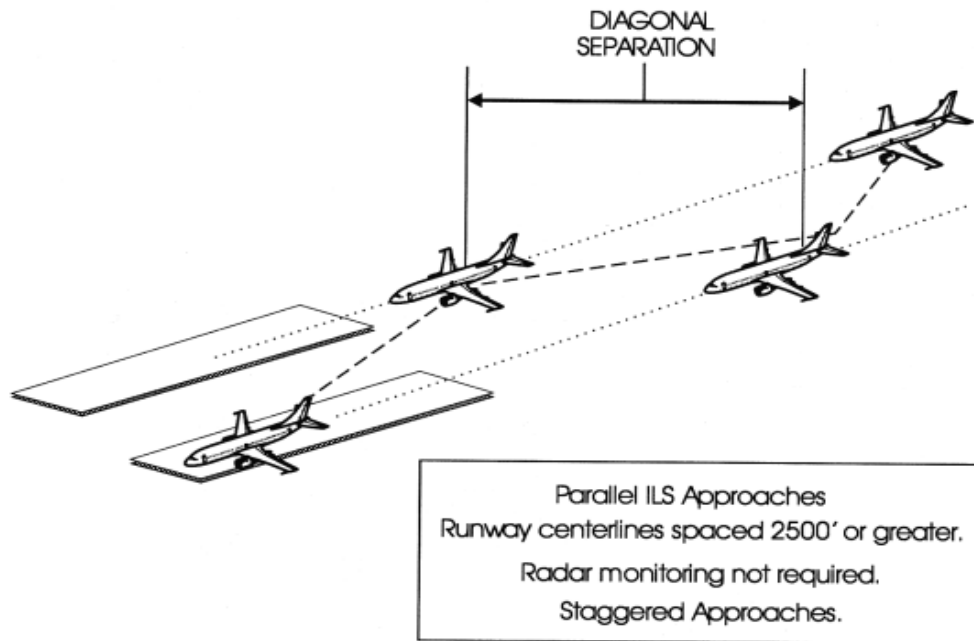
FIG 5-4-16 Staggered ILS Approaches
