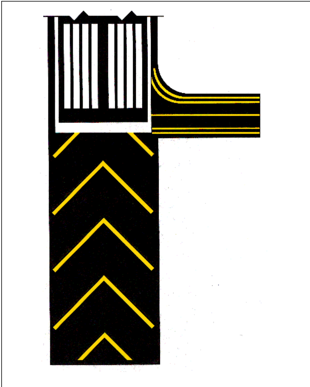
FIG 2-3-8 Enhanced Taxiway Centerline
