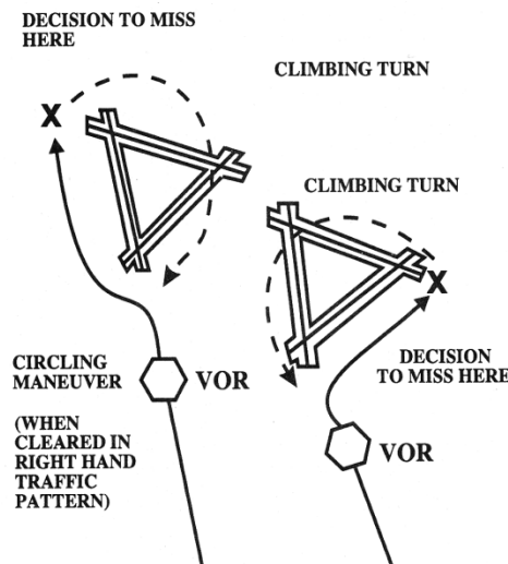
FIG 5-4-26 Missed Approach
