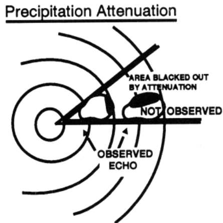
FIG 4-5-1 Limitations to Radar Service
