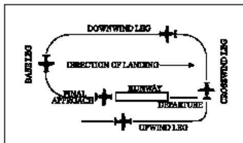
FIG 4-3-1 Components of a Traffic Pattern
