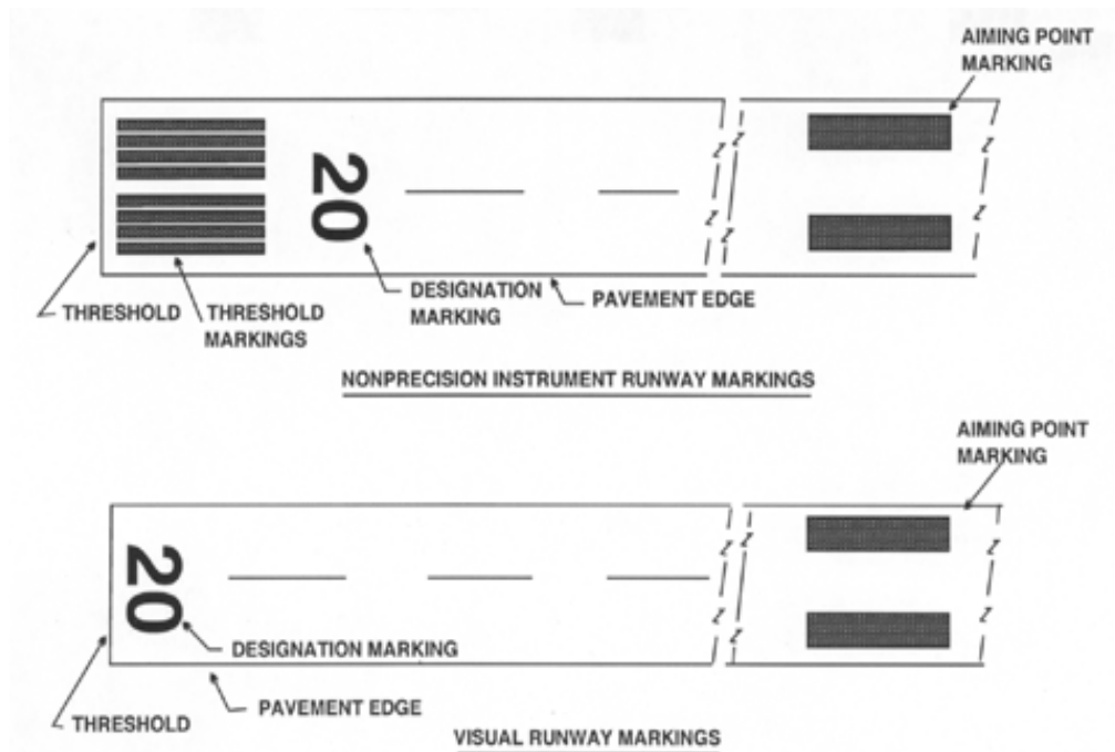
FIG 2-3-2 Nonprecision Instrument Runway and Visual Runway Markings
