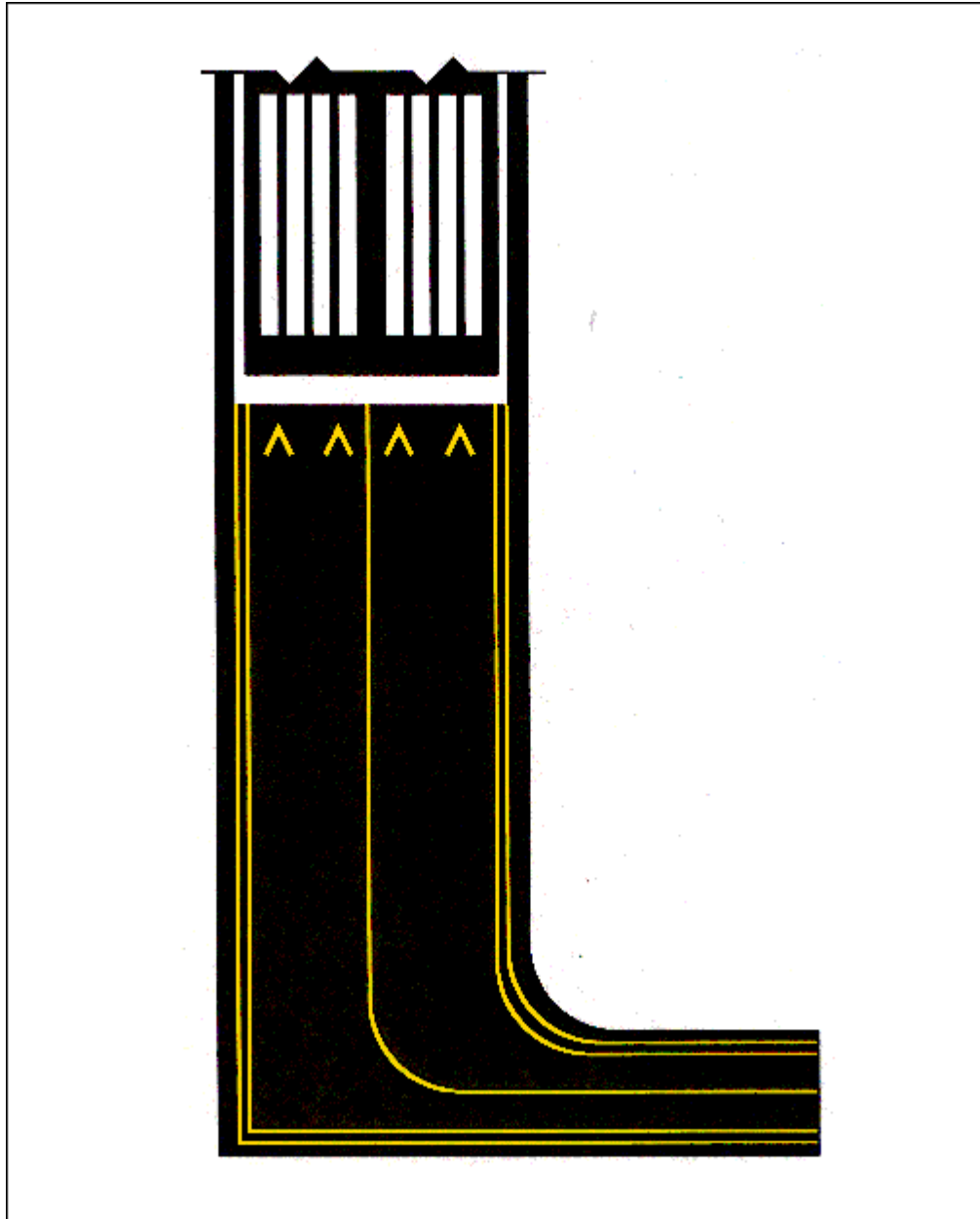
FIG 2-3-4 Displaced Threshold Markings
