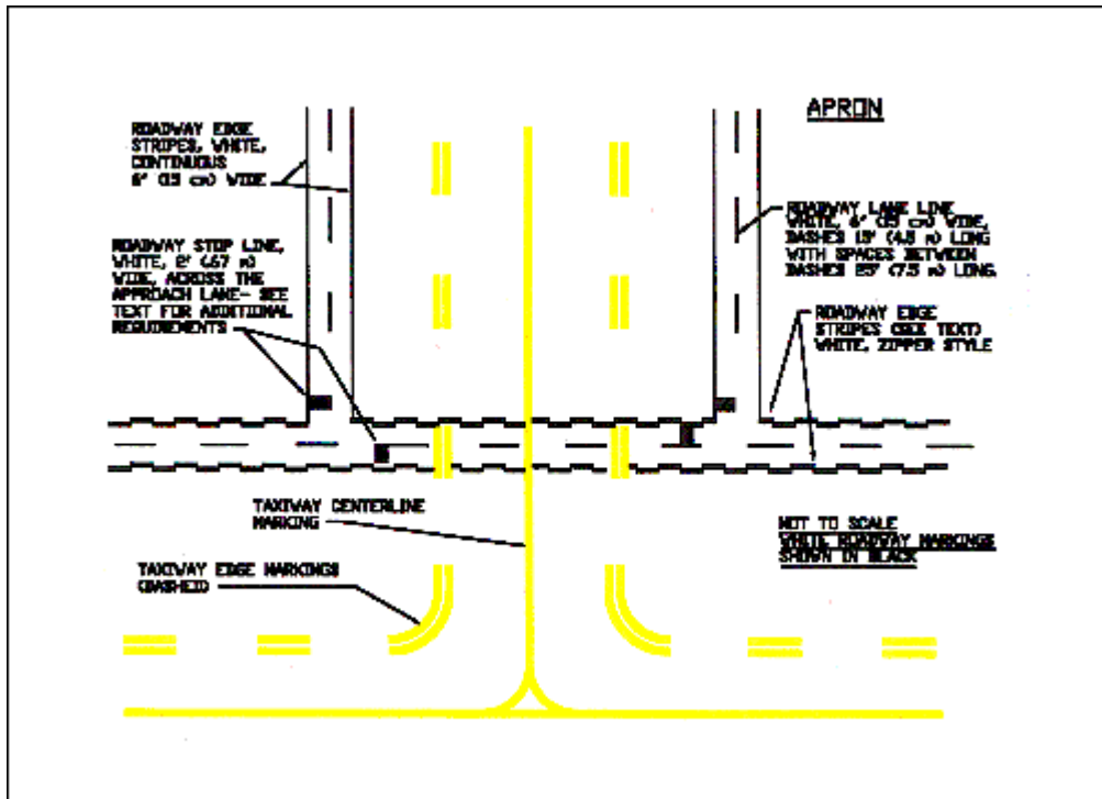
FIG 2-3-19 Roadway Edge Stripes, White, Zipper Style
