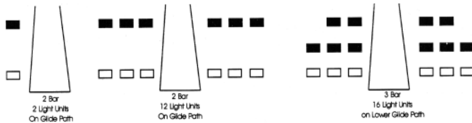
FIG 2-1-4 VASI Variations
