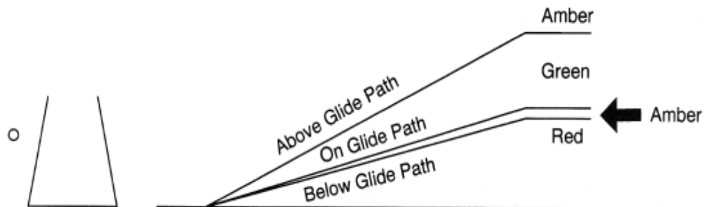
FIG 2-1-6 Tri-Color Visual Approach Slope Indicator
