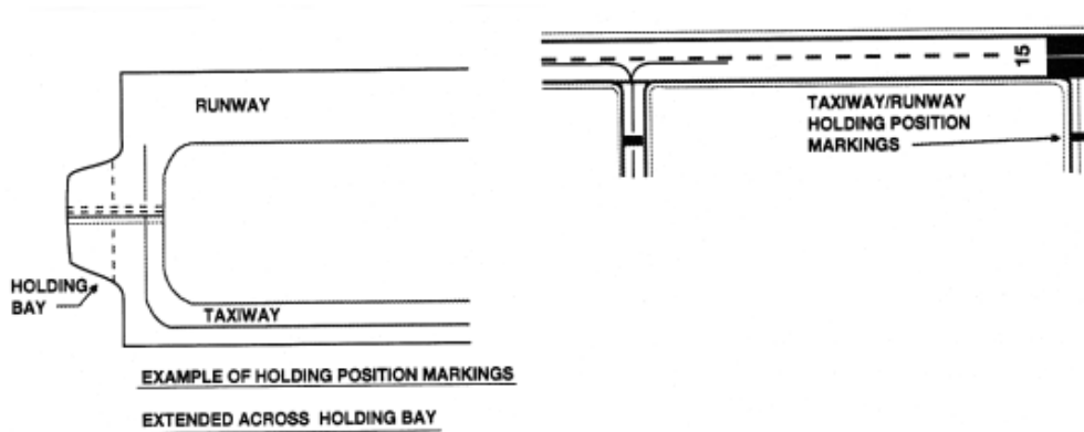
FIG 2-3-14 Runway Holding Position Markings on Runways
