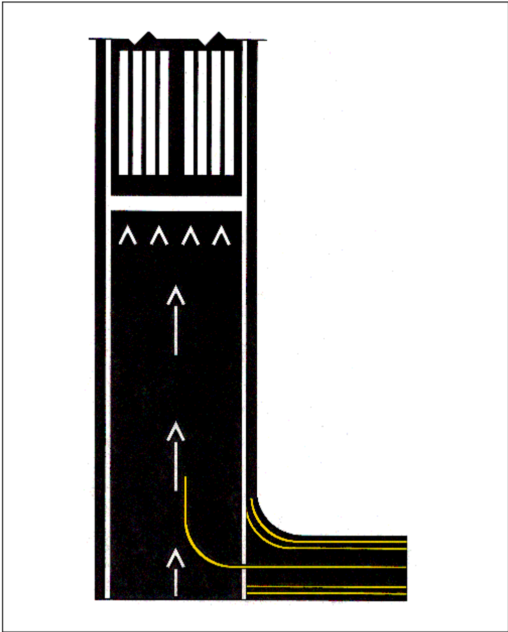
FIG 2-3-5 Runway Shoulder Markings
