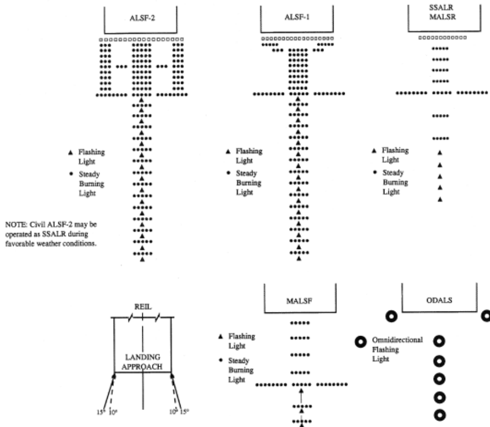
FIG 2-1-1 Precision & Nonprecision Configurations
