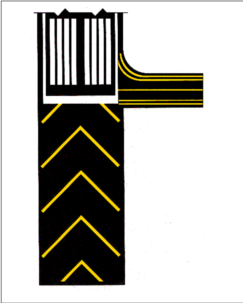
FIG 2-3-8 Enhanced Taxiway Centerline
