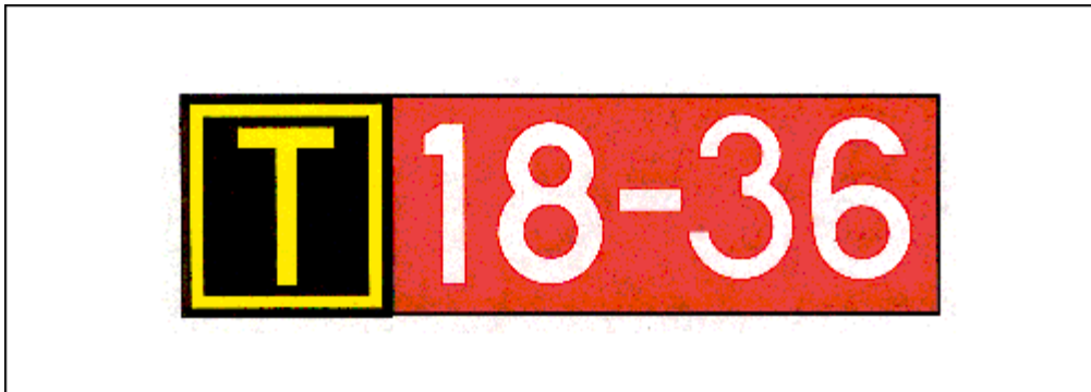
FIG 2-3-31 Taxiway Location Sign Collocated with Runway Holding Position Sign
