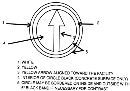
FIG 2-3-21 Nonmovement Area Boundary Markings
